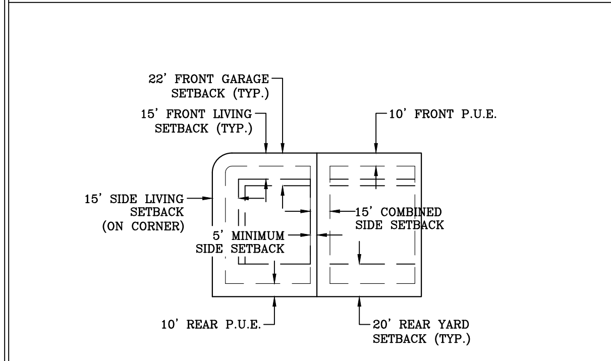
1 TYPICAL EASEMENTS & SETBACKS
