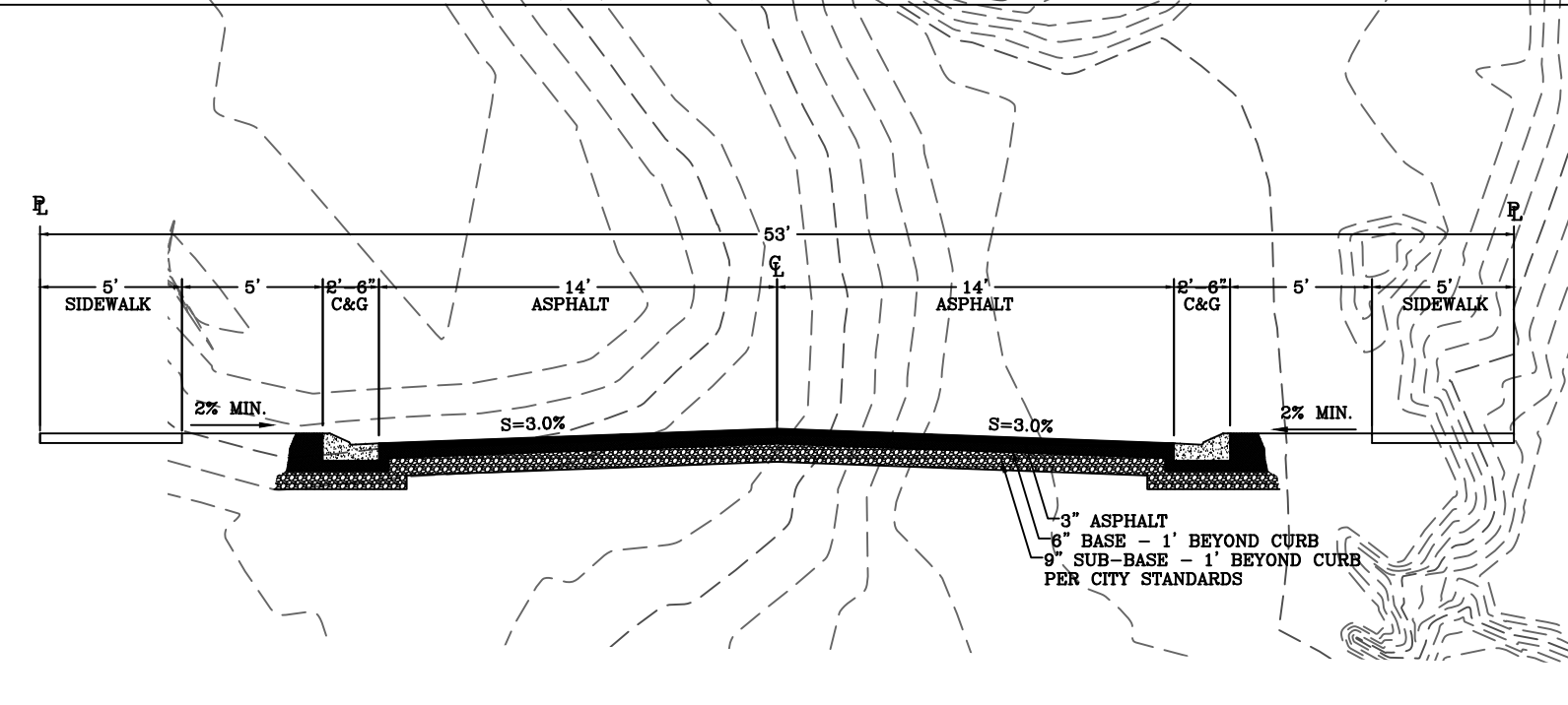
2 53' ROAD CROSS SECTION
